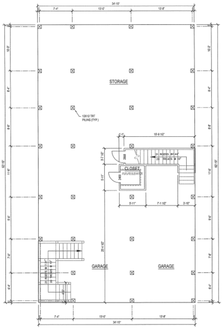
GROUND LEVEL PLAN SCALE: 1/4" = 1'-0"
