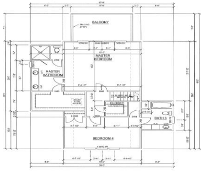
SECOND FLOOR PLAN SCALE: 1/8" = 1'-0"
